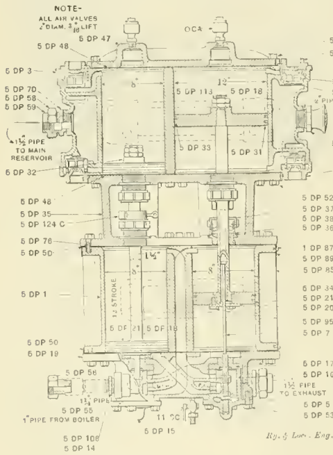
FIG. 1. NEW YORK DUPLEX AIR PUMP, No. 5.
